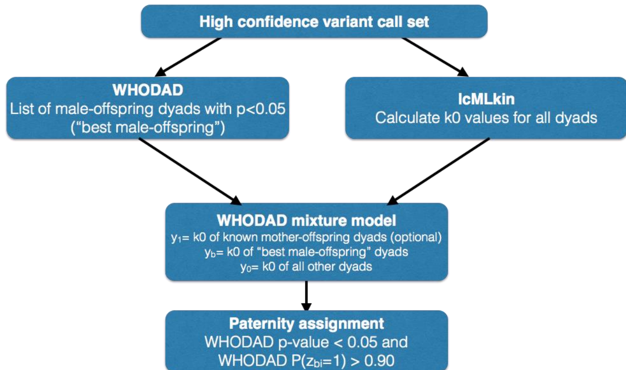
Figure S9 Flowchart for paternity inference using WHODAD. A filtered variant call set is used as input for both WHODAD and lcMLkin (any other relatedness estimation program can also be used). k0 values from lcMLkin are then used to parameterize a mixture model that fits different normal distributions on k0 (corresponding intuitively to different levels of relatedness). By integrating the estimates from the mixture model with the best candidate father from the genotype simulations (used to assign p-values to best candidate fathers), WHODAD then calculates P(z_{bi}=1) , the posterior probability that the best male-offspring dyad is drawn from the distribution of k0 values for parent-offspring pairs. We recommend assigning paternity to candidate father-offspring dyads with a WHODAD p-value < 0.05 and P(z_{bi}=1) > 0.90 . See methods for details.
