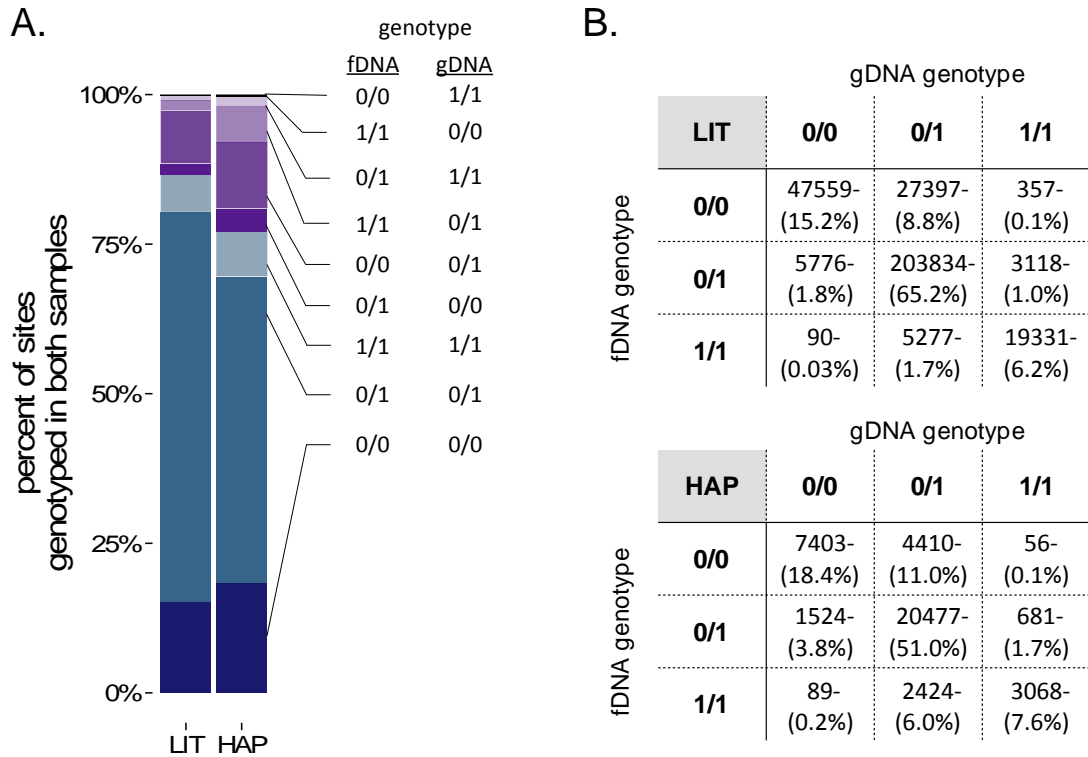
Figure S7 Genotype concordance between paired fDNA and gDNA samples. (A) The fDNA samples captured at least one allele (blue and purple bars) from the paired gDNA samples in 99.8% (LIT) and 99.6% (HAP) of sites genotyped. Paired samples therefore had completely discordant genotypes (0/0 and 1/1 or 1/1 and 0/0; black and dark grey bars) in less than 0.5% of genotyped sites. The 9 possible combinations of genotype calls in paired fDNA (first column) and gDNA samples (2 nd column) are shown to the right of the stacked barcharts; in all cases, the reference allele is represented as 0 and the alternate allele as 1. (B) Table of genotype concordance/discordance rates between sites genotyped in paired fDNA and gDNA libraries. The top table shows the results for LIT fDNA-gDNA and the bottom table for HAP fDNA-gDNA.
